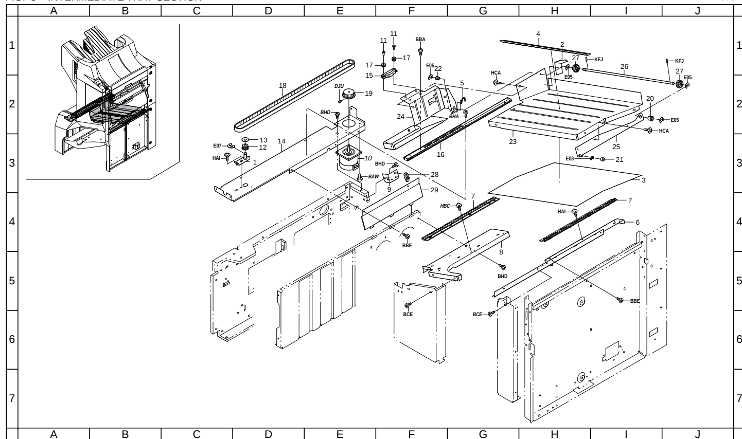
FIG. 8 INTERMEDIATE TRAY SECTION
