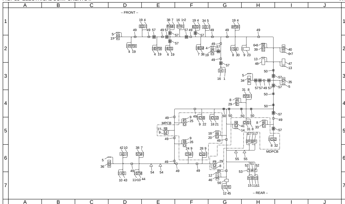
FIG. 13 ELECTRICAL COMPONENTS II
