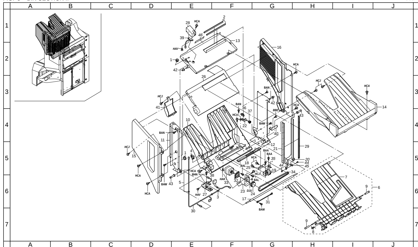
FIG. 5 BIN SECTION II
