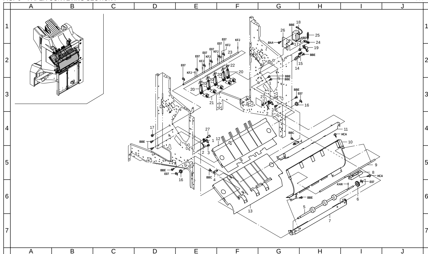
FIG. 6 PAPER CONVEYING SECTION I
