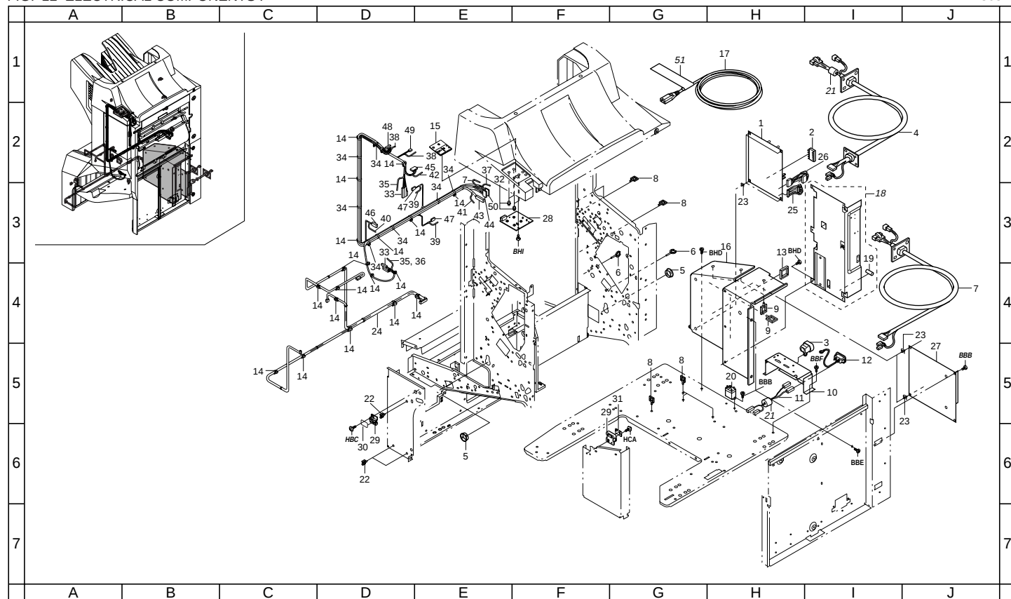
FIG. 12 ELECTRICAL COMPONENTS I
