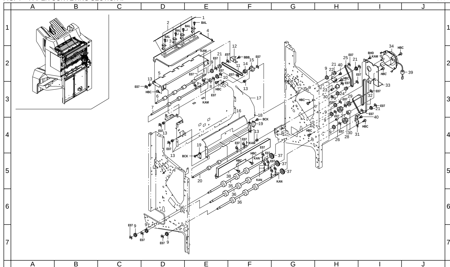
FIG. 7 PAPER CONVEYING SECTION II
